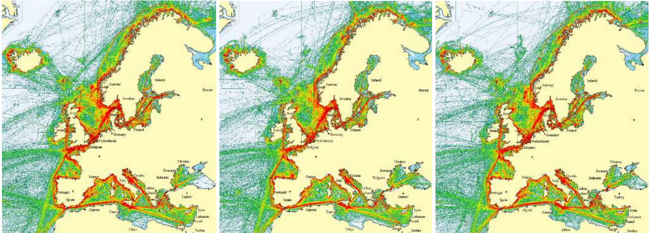
Figure 8: All ship types: ship traffic density in June 2019 (left), in June 2020 (centre) and in June 2021 (right)
